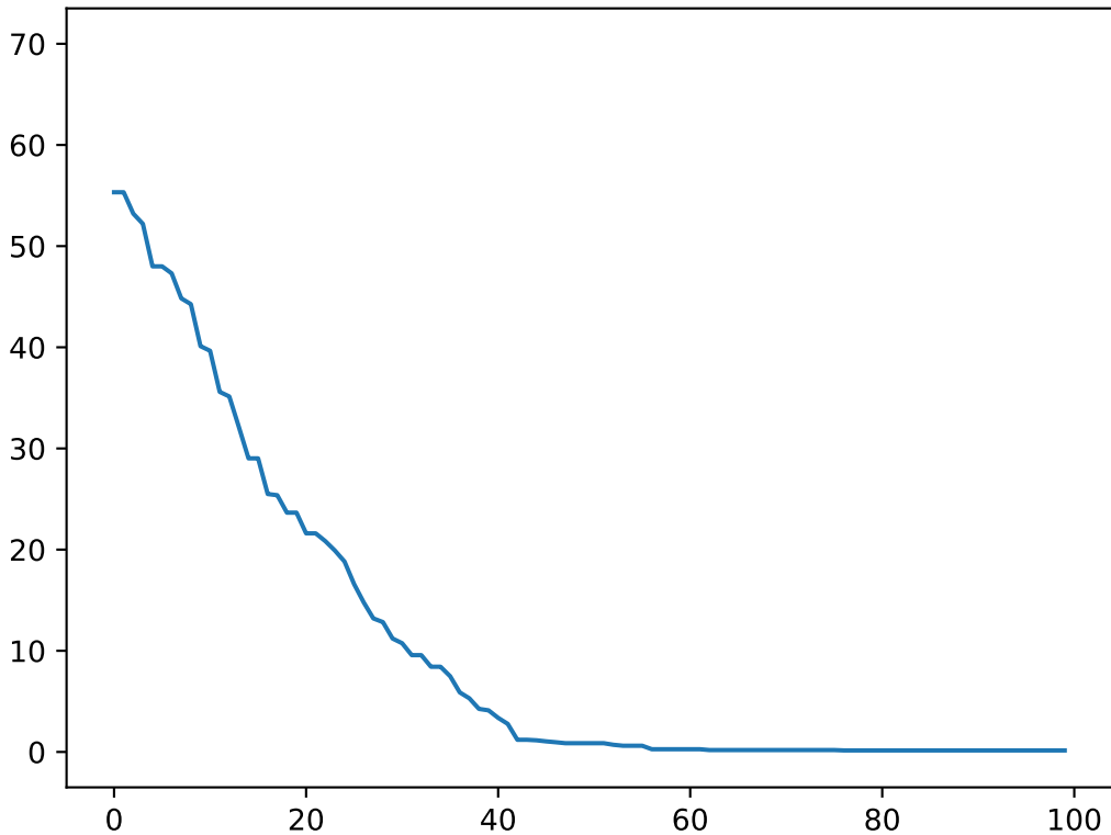
Best-of-Generation Fitness
