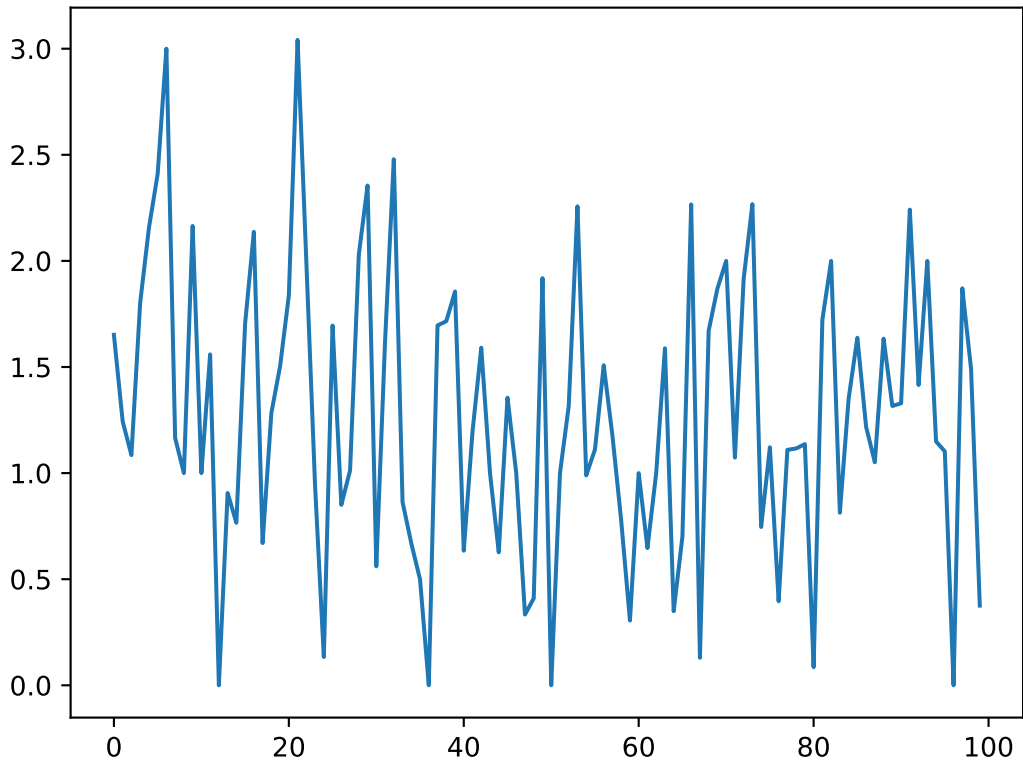
Best-of-Generation Fitness
