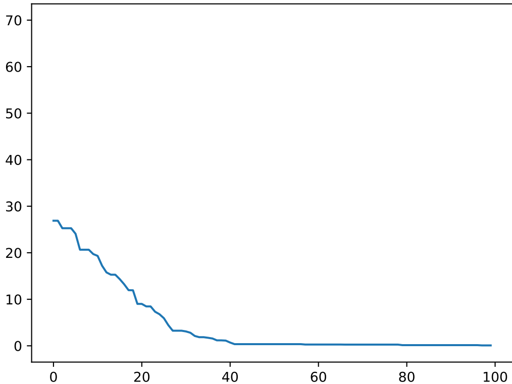
Best-of-Generation Fitness
