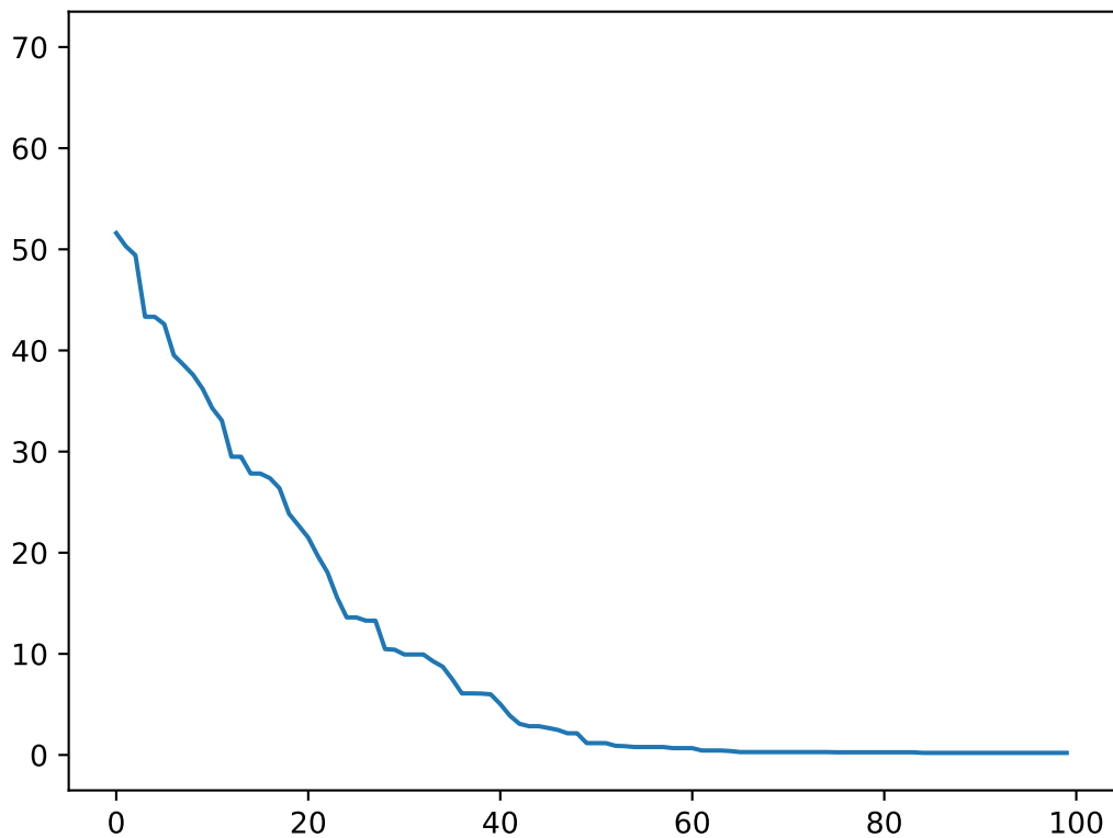
Best-of-Generation Fitness
