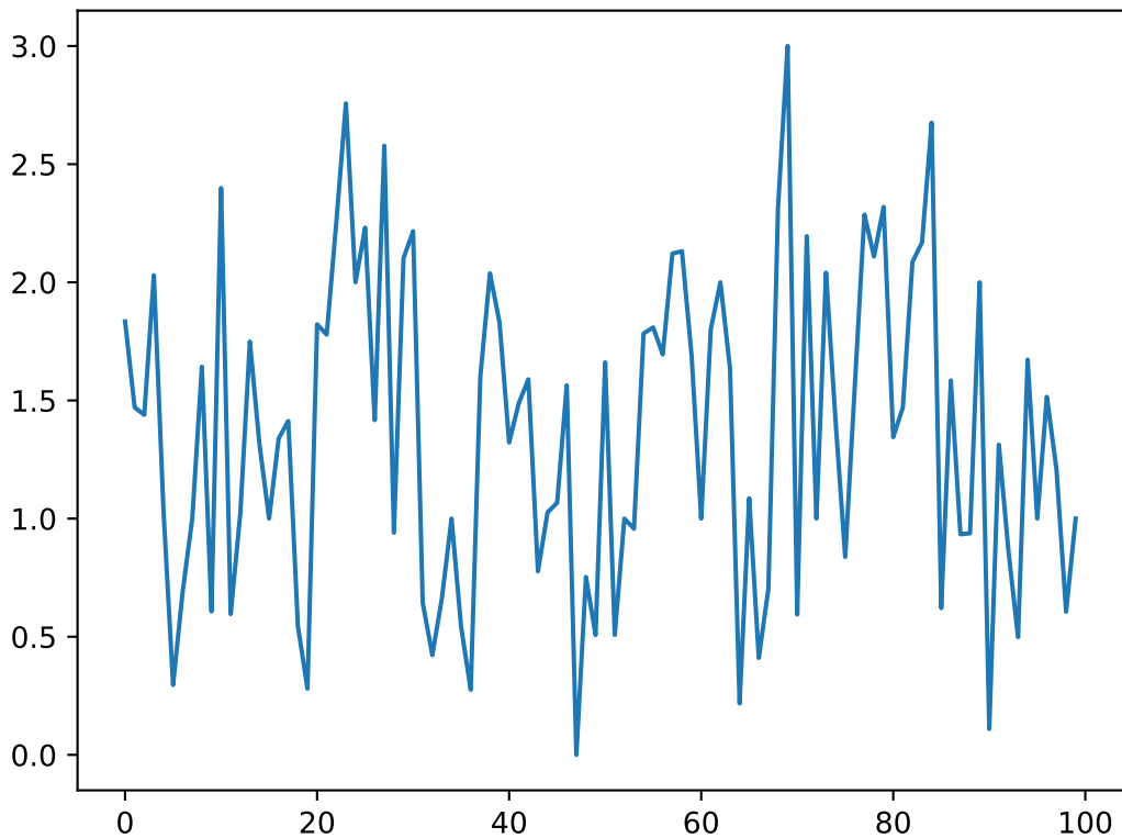
Best-of-Generation Fitness
